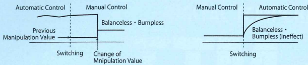
BALANCELESS · BUMPLESS
