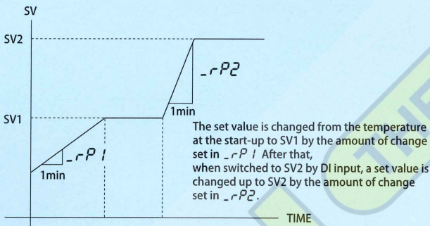
SV2 is switched by DI input communication key.
